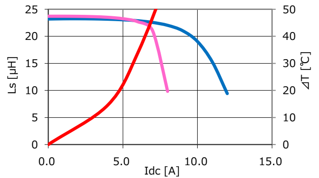
CDEP15D90T150NP-220MC-100
