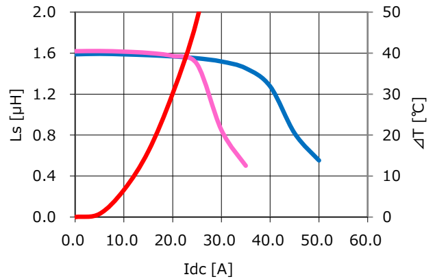
CDEP15D90T150NP-1R6MC-100
